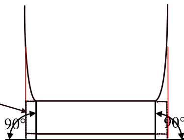
View of heel from the rear of the shoe (Type A and B)
